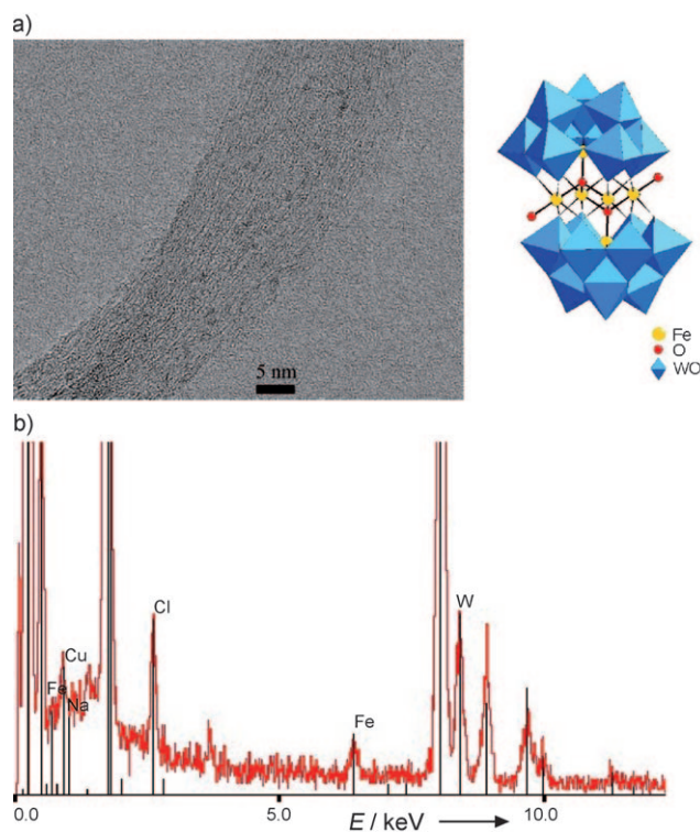
Figure 1. a) HRTEM image of bundles of nanotubes decorated by \text{Fe}_6 -POM and view of the structure of the polyoxoanion [\text{Fe}_4(\text{H}_2\text{O})_2(\text{FeW}_9\text{O}_{34})_2]^{10-} ; b) the EDX spectrum of the \text{Fe}_6 @NT system. The red curve is the experimental spectrum; the black lines show the energy of each band of the spectrum.
